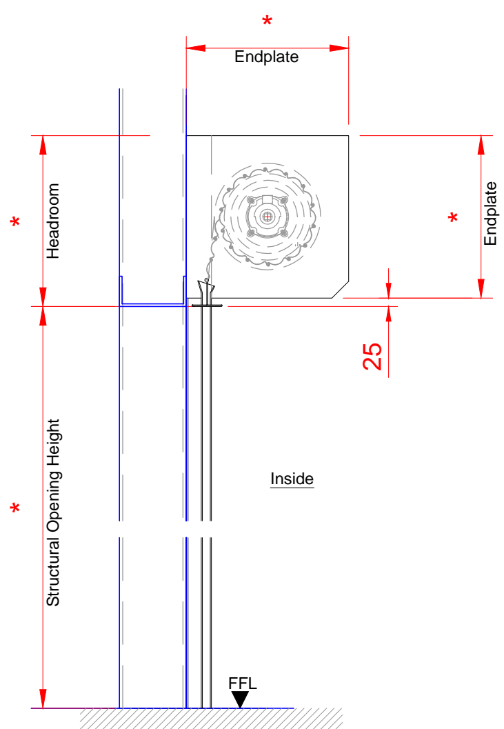
SECTION
