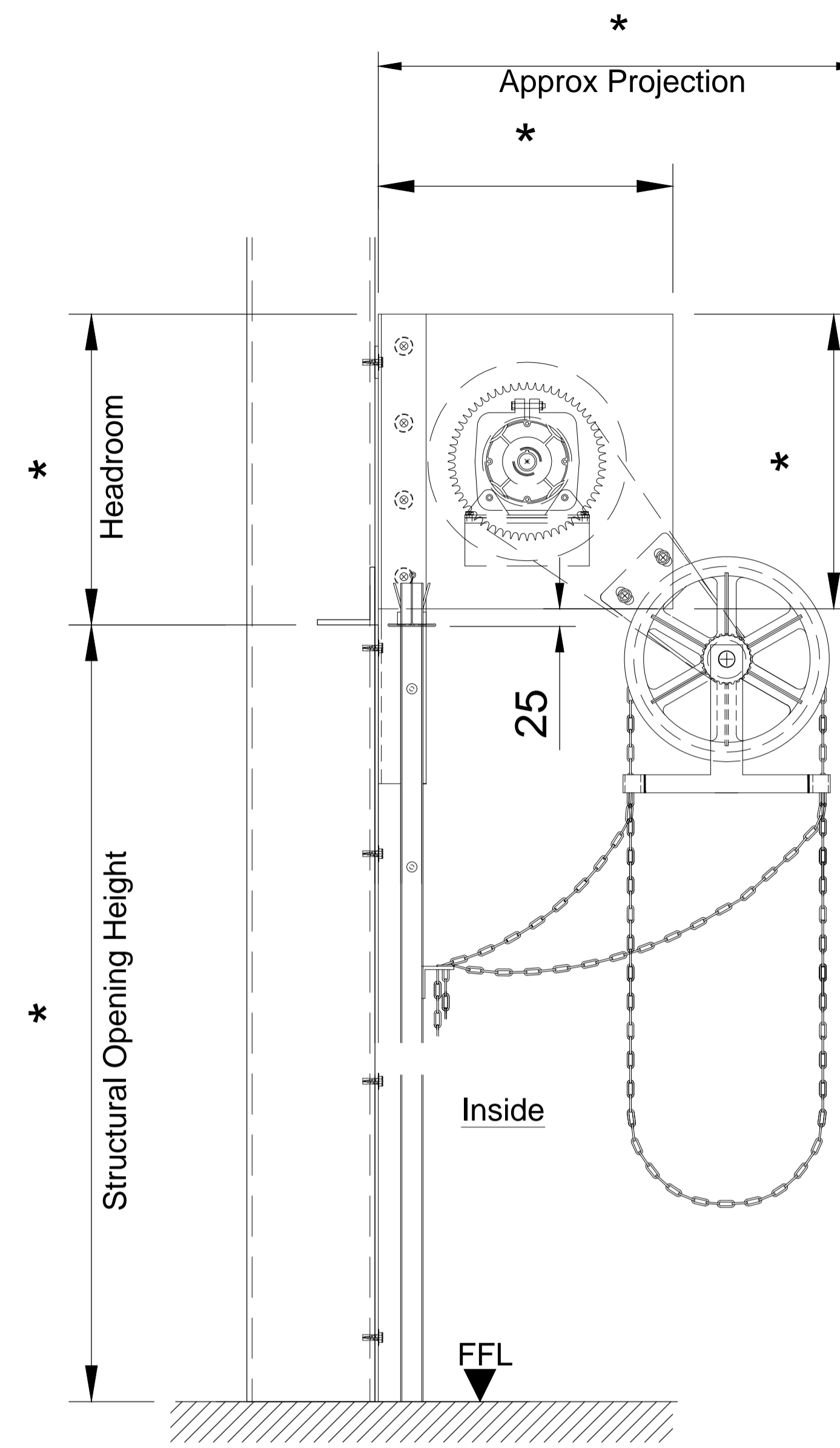
SECTION
